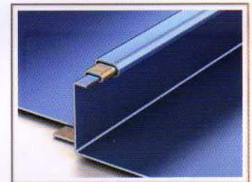
Premium Lock 150 1.5" Standing Seam Also available in 1"
